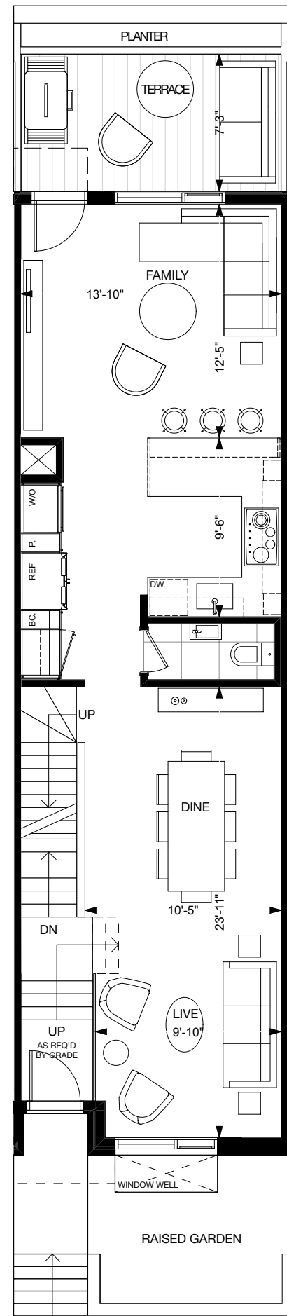
MAIN LEVEL ELEV. 'A'
