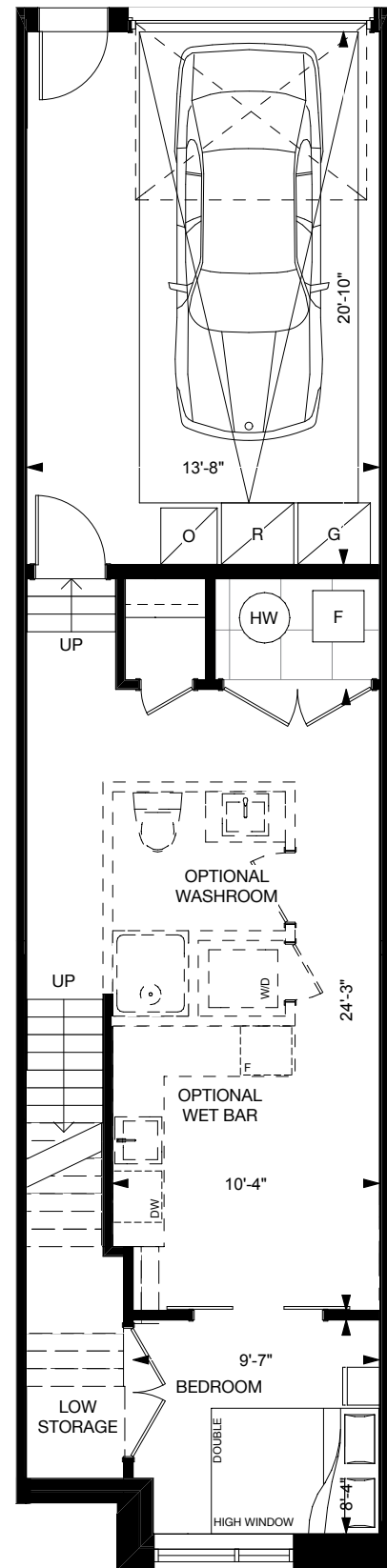
GROUND LEVEL ELEV. 'A'
