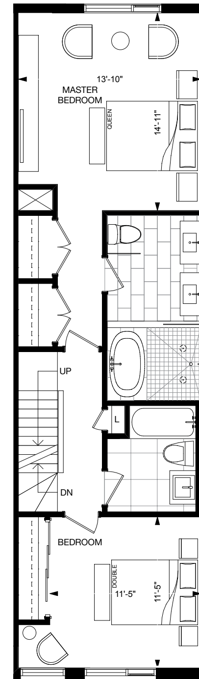
SECOND LEVEL ELEV. 'A'
